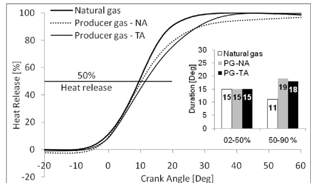
Fig. 1 – Heat release profile and duration for producer gas and natural gas.
